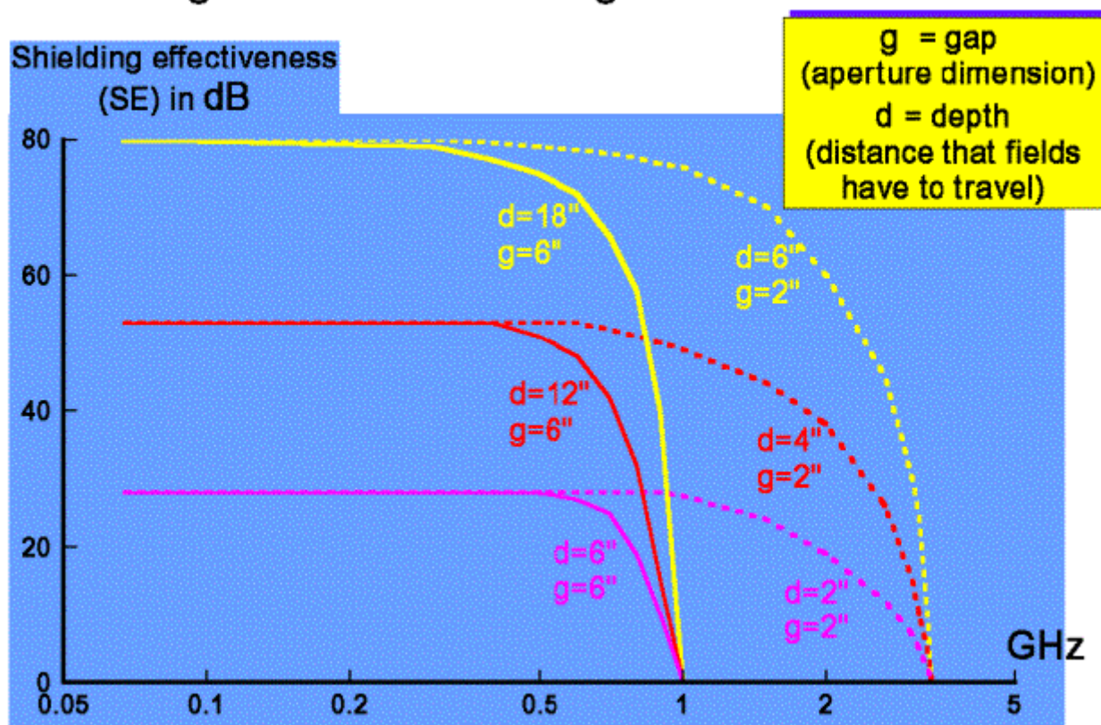
Figure 4J Some waveguides below cut-off
