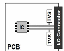
Good PCB Layout
