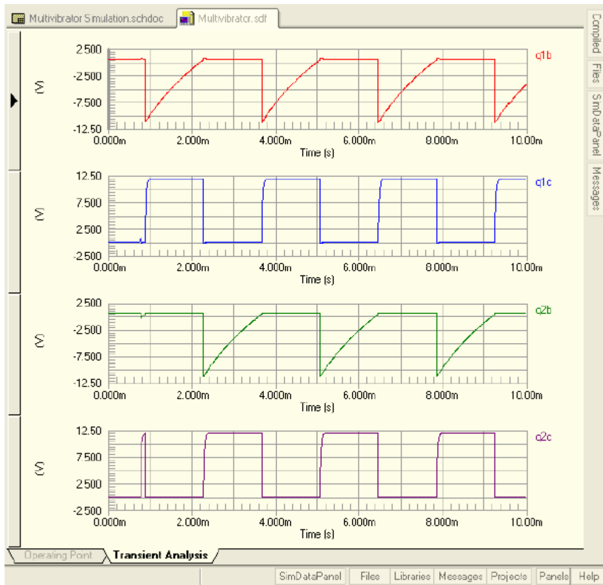
Figure 10. Output waveforms from the multivibrator.
