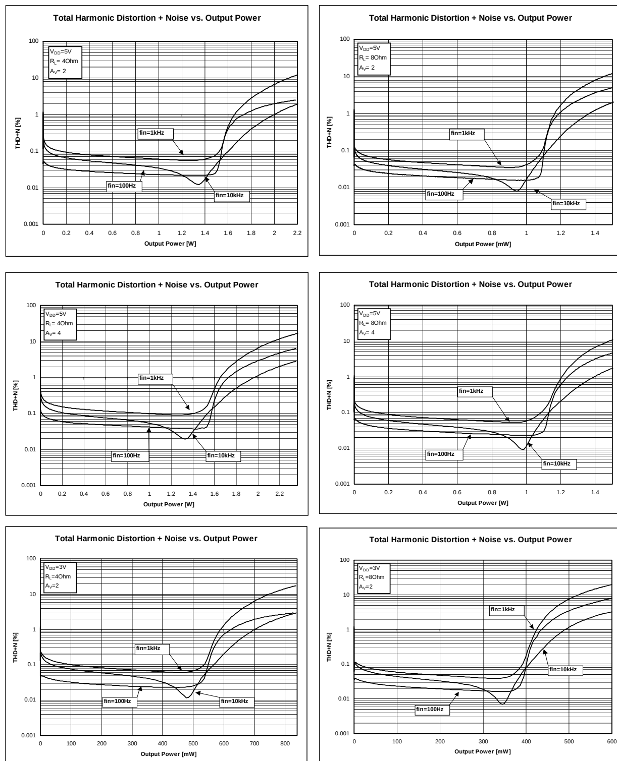
Figure 3. Total Harmonic Distortion – Noise vs. Output Power
