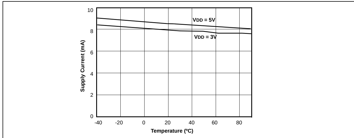
Figure 9. Supply Current vs. Temperature
