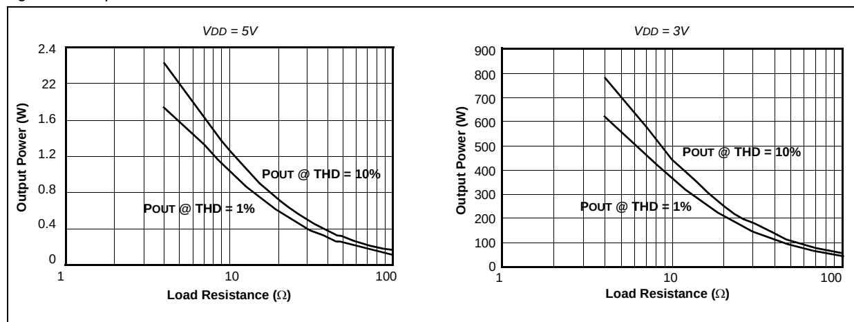
Figure 6. Output Power vs. Load Resistance
