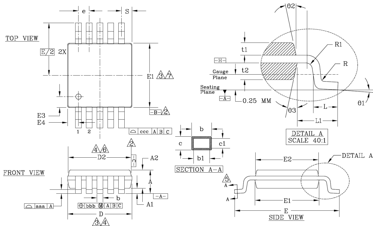
Figure 17. MSOP-10 Package
