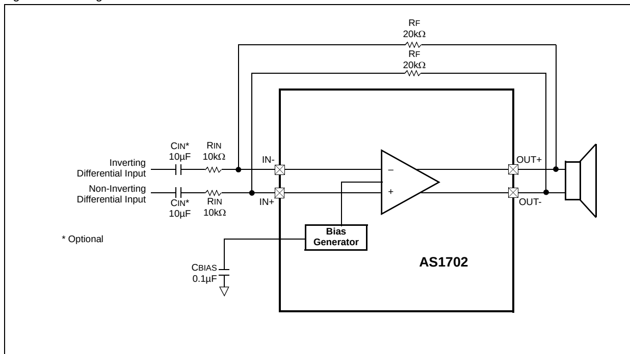
Figure 15. Setting the AS1702 Gain
