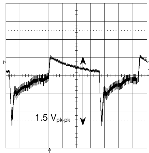
Figure 29 - Transient Response 130 V AC 50 Hz, I_{OUT} : 0 A to 1.83 A V_{OUT} (200 mV, 5ms/div)
