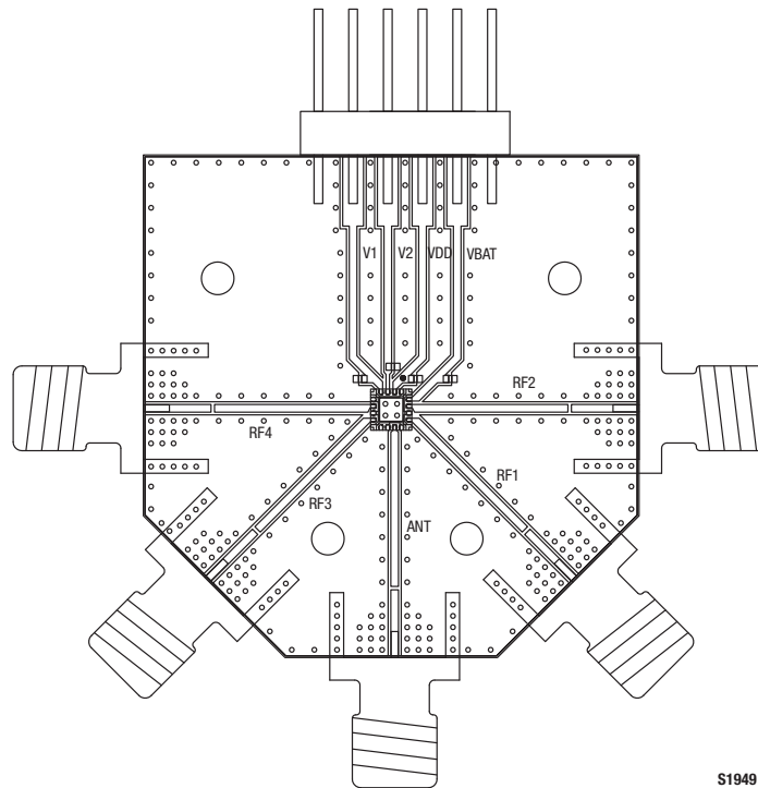
Figure 13. SKY14151-350LF Evaluation Board Assembly Diagram
