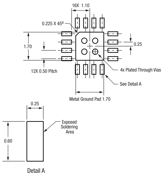
Figure 14. SKY14151-350LF PCB Layout Footprint (Top View)
