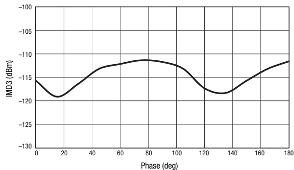
Figure 9. 3 rd Order Intermodulation Distortion vs Phase
