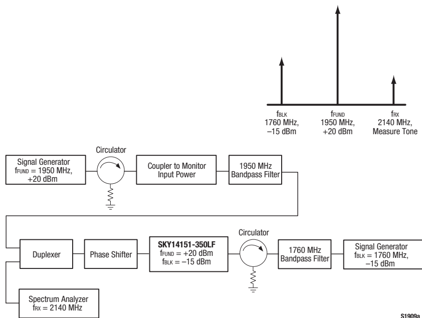
Figure 10. 3 rd Order Intermodulation Test Setup
