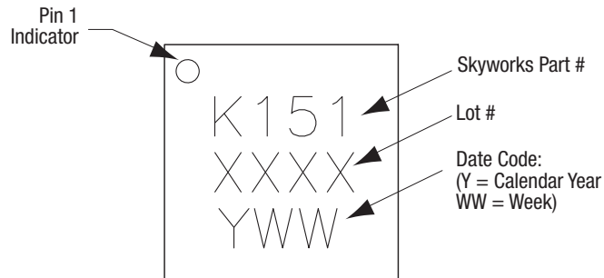
Figure 15. Typical Case Markings (Top View)
