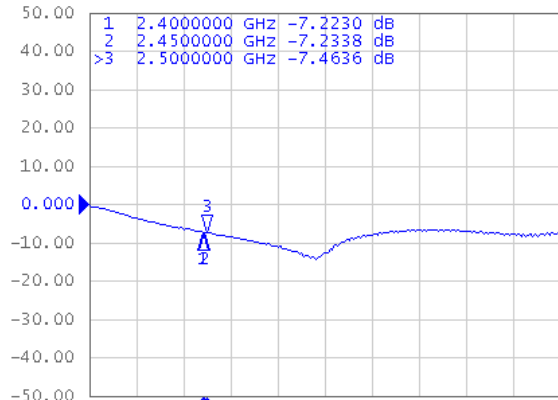
Tr3 S12 Log Mag 10.00dB/ Ref 0.000dB [F2]
