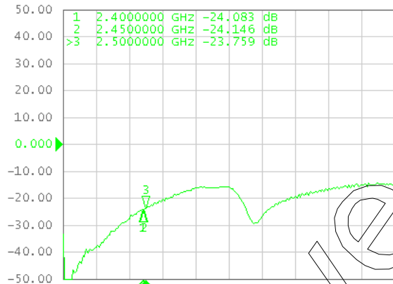
Tr3 S12 Log Mag 10.00dB/ Ref 0.000dB [F2]
