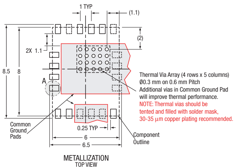
Figure 4. Phone PCB Layout Footprint for 6 x 8 mm, 20-Pad Package with Grid-Bottom Solder Mask – SKY77518 Specific.
