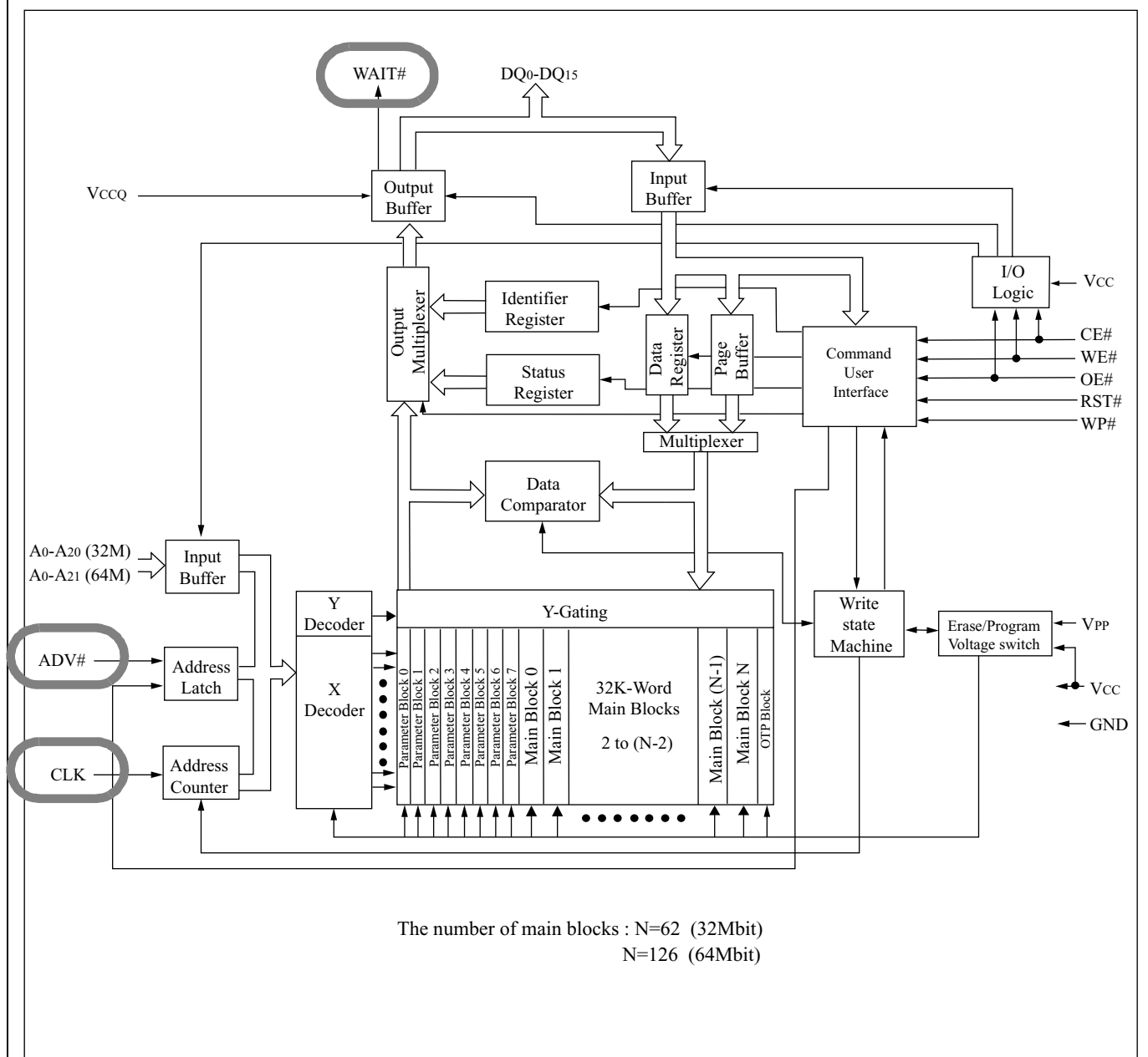
Figure 1. Block Diagram
