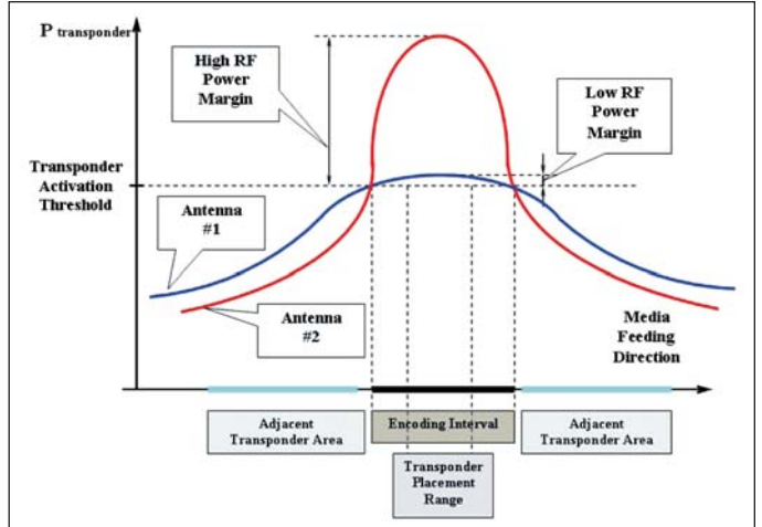
Figure 3 · Power delivered to a transponder and RF power margin.
