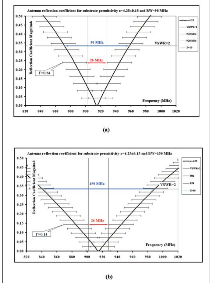
Figure 4 · Antenna reflection coefficient and impedance bandwidth ( BW ). (a) BW = 90 MHz; (b) BW = 150 MHz.
