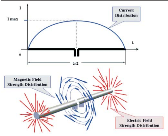
Figure 2 · Dipole current distribution and fields.
