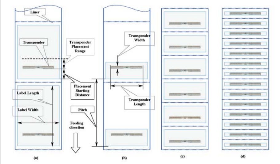
Figure 1 · Smart Label structure and transponder placement. (a) Smart Label design; (b) short labels with long pitch; (c) short Smart Labels; (d) small labels with short pitch.
