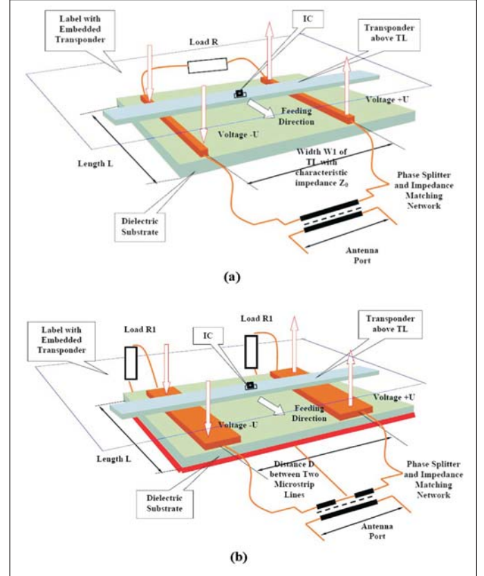
Figure 7 . Antennas based on Terminated Non-Resonant TL. (a) “Two-Wire” transmission line; (b) “Dual Microstrip” transmission line.
