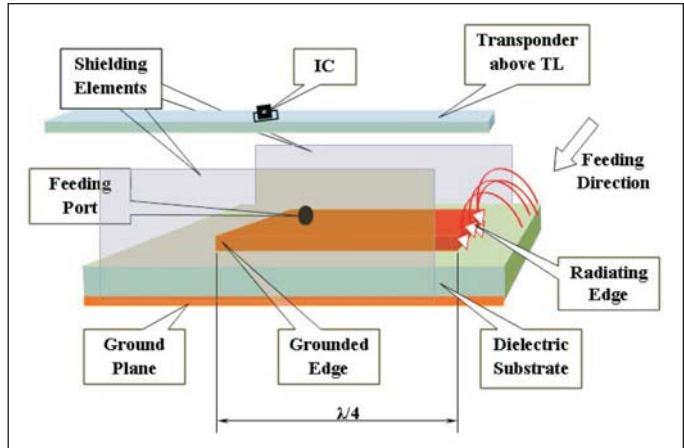
Figure 6 · Open Transmission Line antenna— \lambda/4 wavelength microstrip patch.
