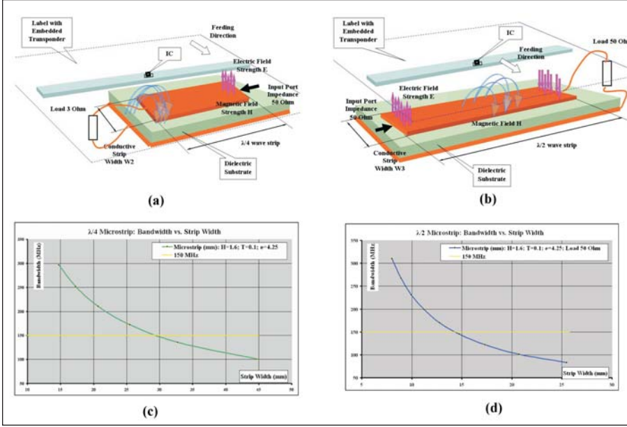
Figure 8 · Antennas based on Terminated Uniform Resonant microstrip TL for 915 MHz band. (a) \lambda/4 TL antenna; (b) \lambda/2 TL antenna; (c) \lambda/4 TL bandwidth vs. width; (d) \lambda/2 TL antenna bandwidth vs. width.
