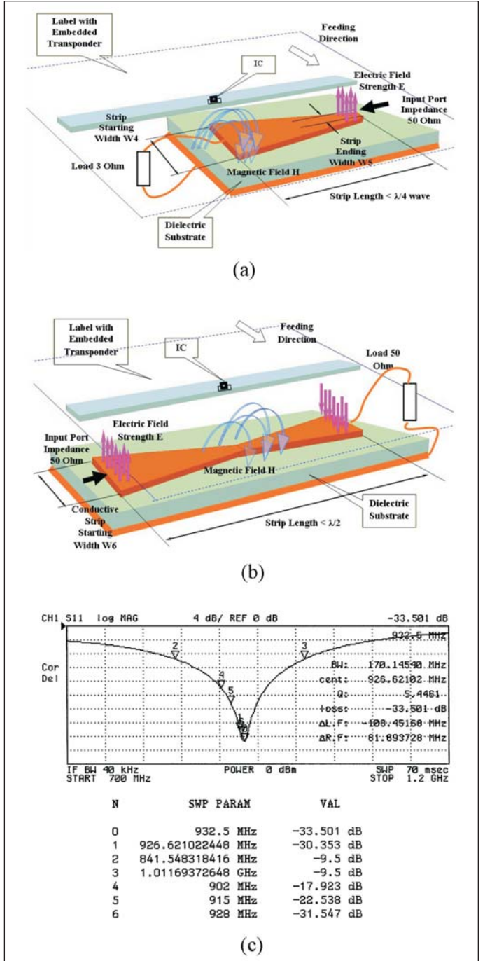
Figure 9 · Antennas based on Terminated Tapered Resonant microstrip TL: (a) \lambda/4 TL antenna; (b) \lambda/2 TL antenna; (c) S_{11} parameter for \lambda/2 TL antenna dimensions 4.5 \times 18 \times 65 mm.
