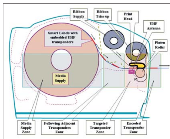
Figure 5 · Common architecture of thermal transfer UHF RFID Printer-Encoder.
