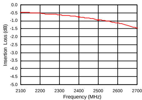
Insertion Loss
