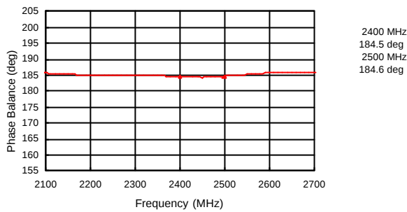
Phase Balance
