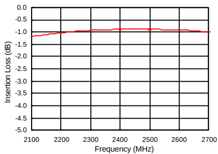
Insertion Loss
