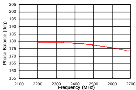
Phase Balance
