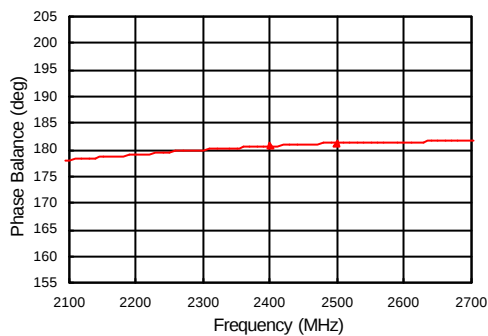
Phase Balance
