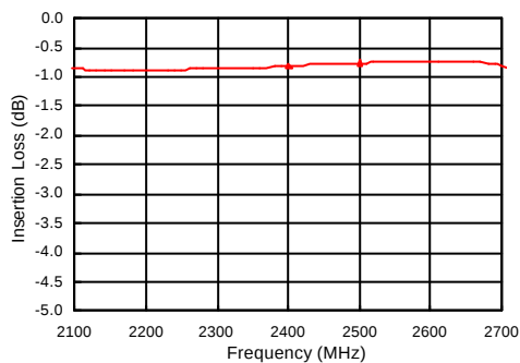
Insertion Loss
