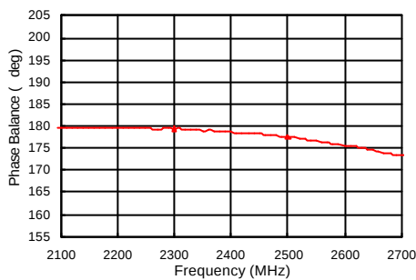
Phase Balance
