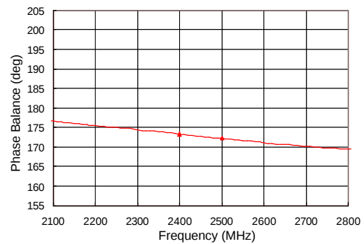
Phase Balance
