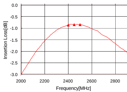
Insertion Loss
