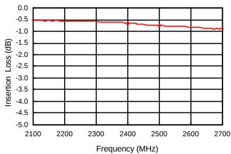
Insertion Loss
