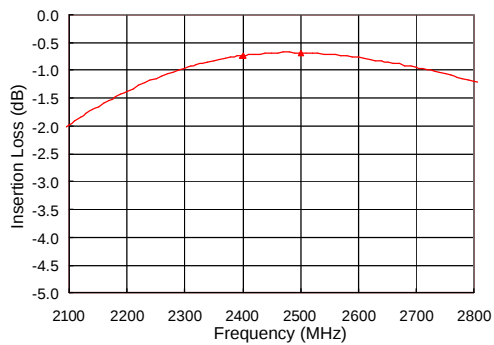
Insertion Loss
