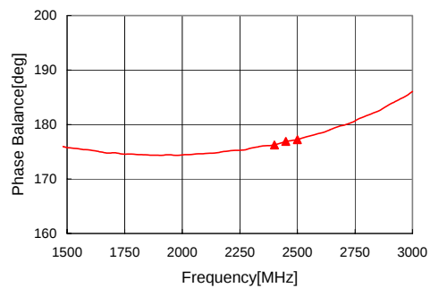
Phase Balance
