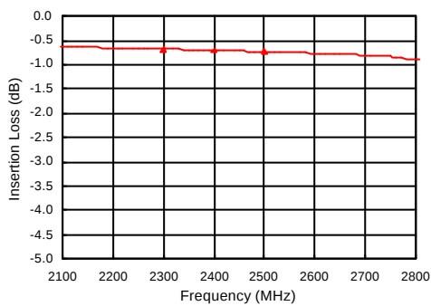
Insertion Loss
