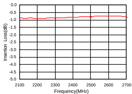
Insertion Loss
