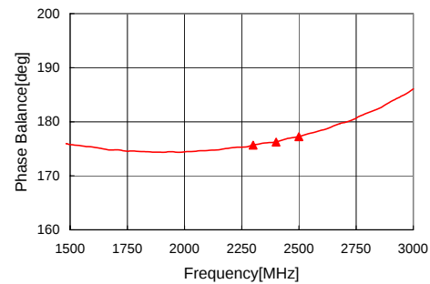
Phase Balance
