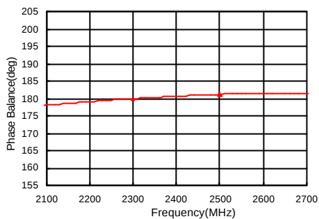
Phase Balance
