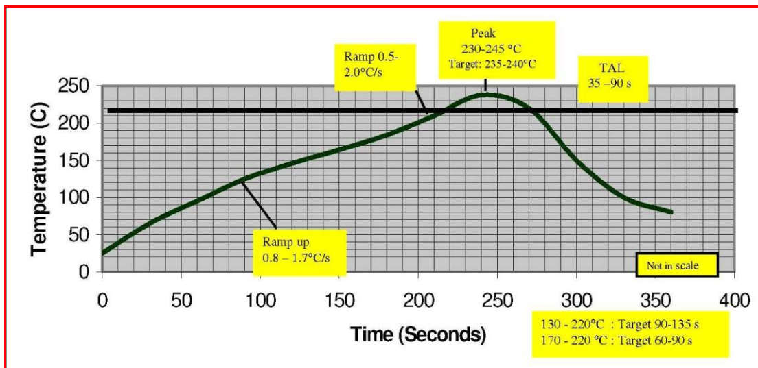
Figure 5: Reflow Profile
