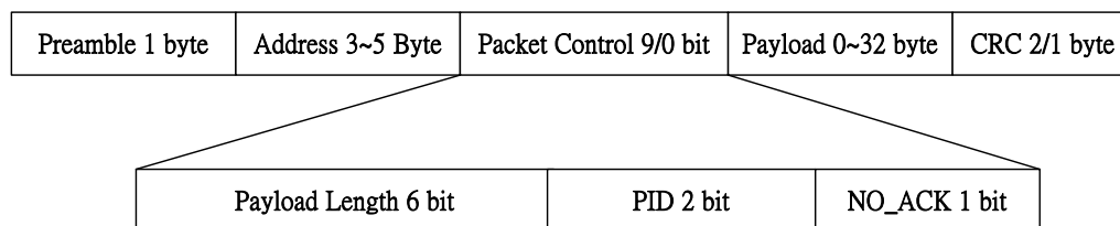
Fig 3, Packet format
