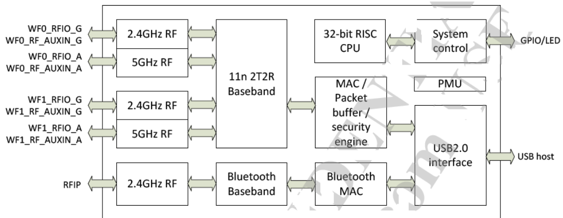
Figure 1 MT7632U block diagram
