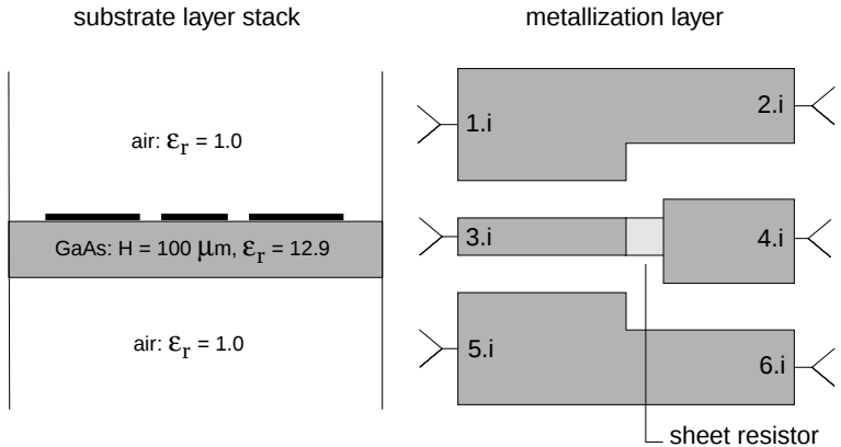
Figure A-13. CPW step-in-width with integrated sheet resistor
