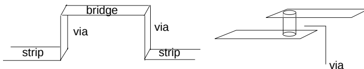
Examples of vias as sheets and cylinders
