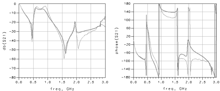
Figure A-12. Magnitude and phase of S21. The thicker line is Momentum results, the thinner line is the measurement.
