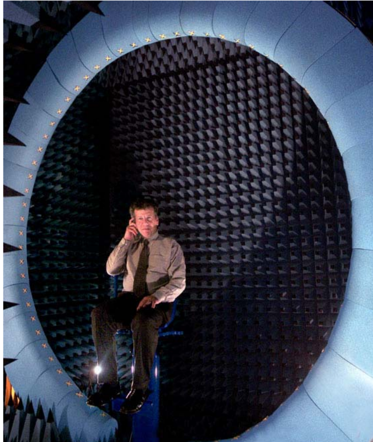
Spherical near-field chamber at Philips Research Laboratories
